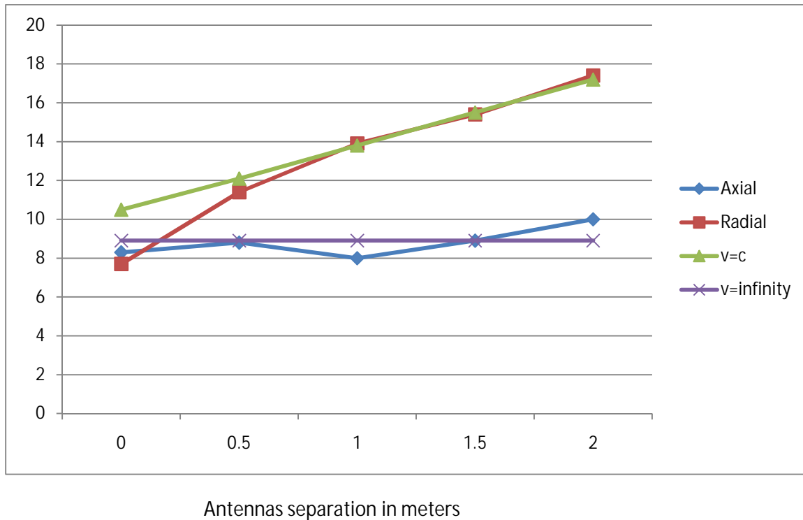
Figure 2. Differential delay as a function of transmitter-receiver separation
